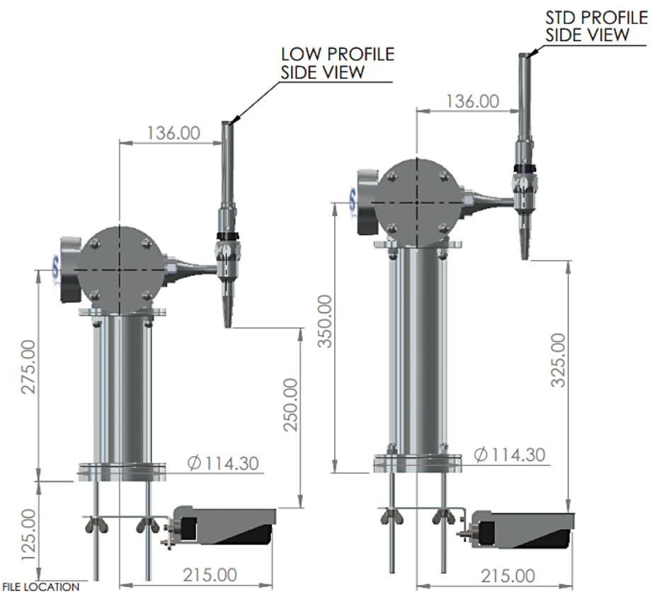
ARTISAN BRIDGE T BAR FONT [ T.B , FRONT MOUNT]
