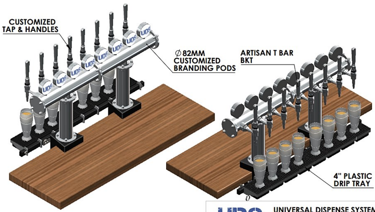
ARTISAN BRIDGE T BAR FONT [BKT , TOP MOUNT]
