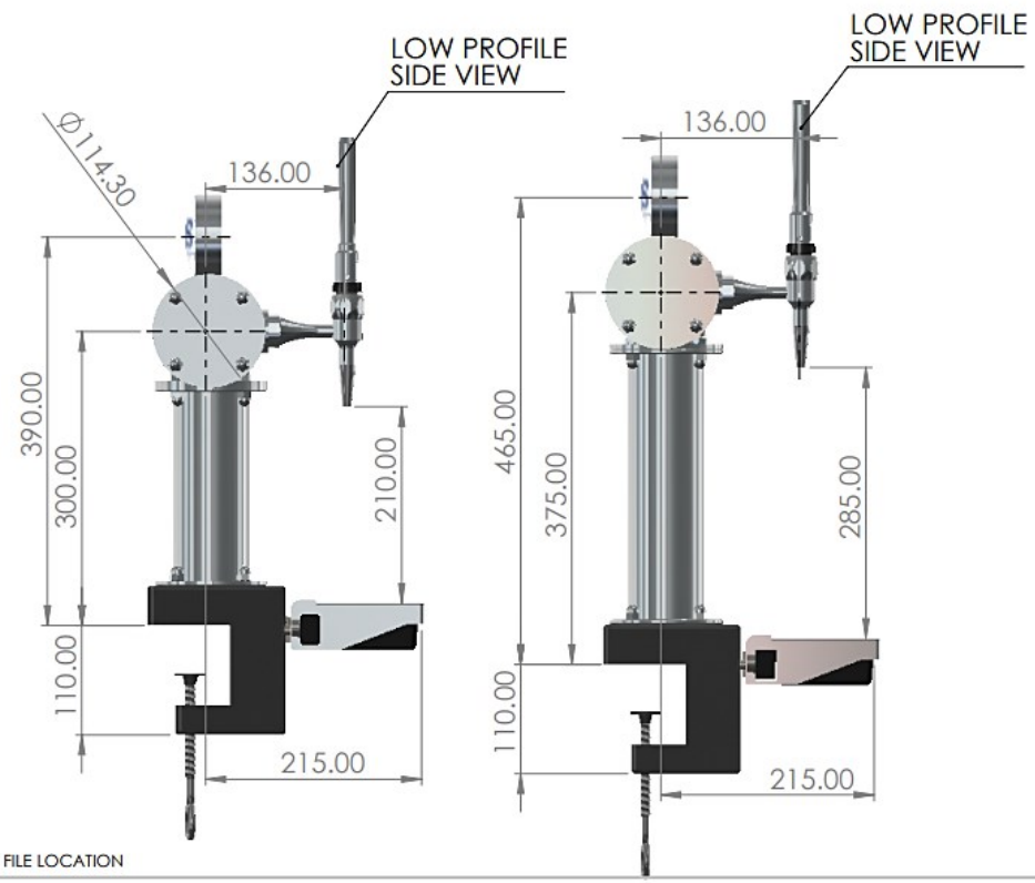
ARTISAN BRIDGE T BAR FONT [BKT , TOP MOUNT]
