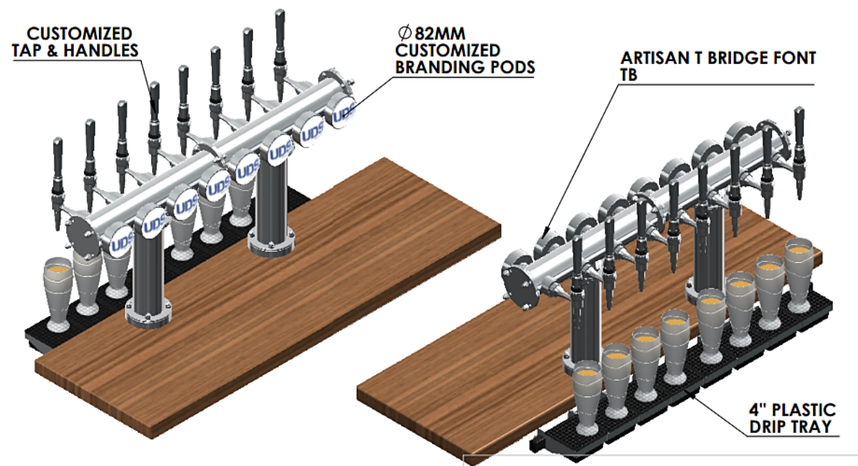
ARTISAN BRIDGE T BAR FONT [ T.B , FRONT MOUNT]
