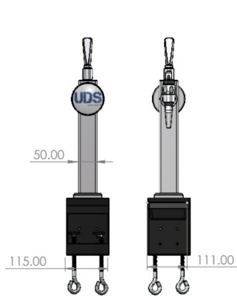
FROTN VIEW BACK VIEW
