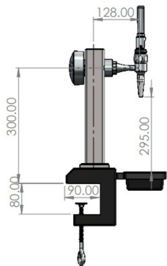
SIDE VIEW (SINGLE)
