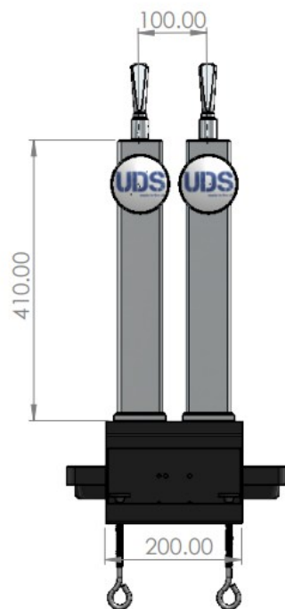
FROTN VIEW
