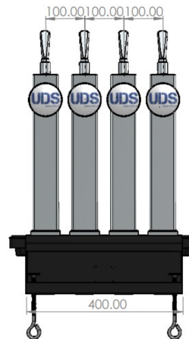
FROTN VIEW
